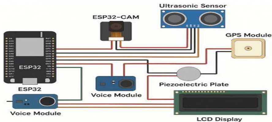
Fig 1: Electrical Design (Circuit Connections for Sensor & Feedback Systems)
